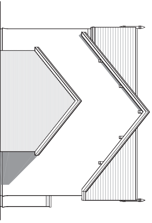
SIDE ELEVATION
